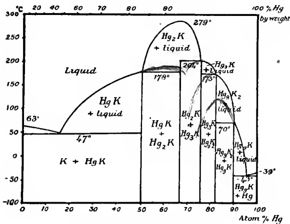
FIG. 15.—Mercury and potassium.
